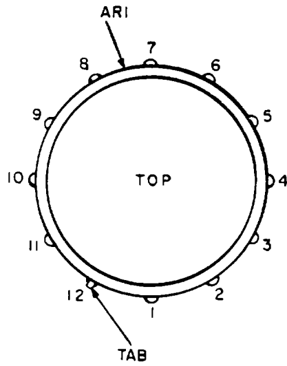
Figure 5-10. Operational amplifier A1AR1 test points.
